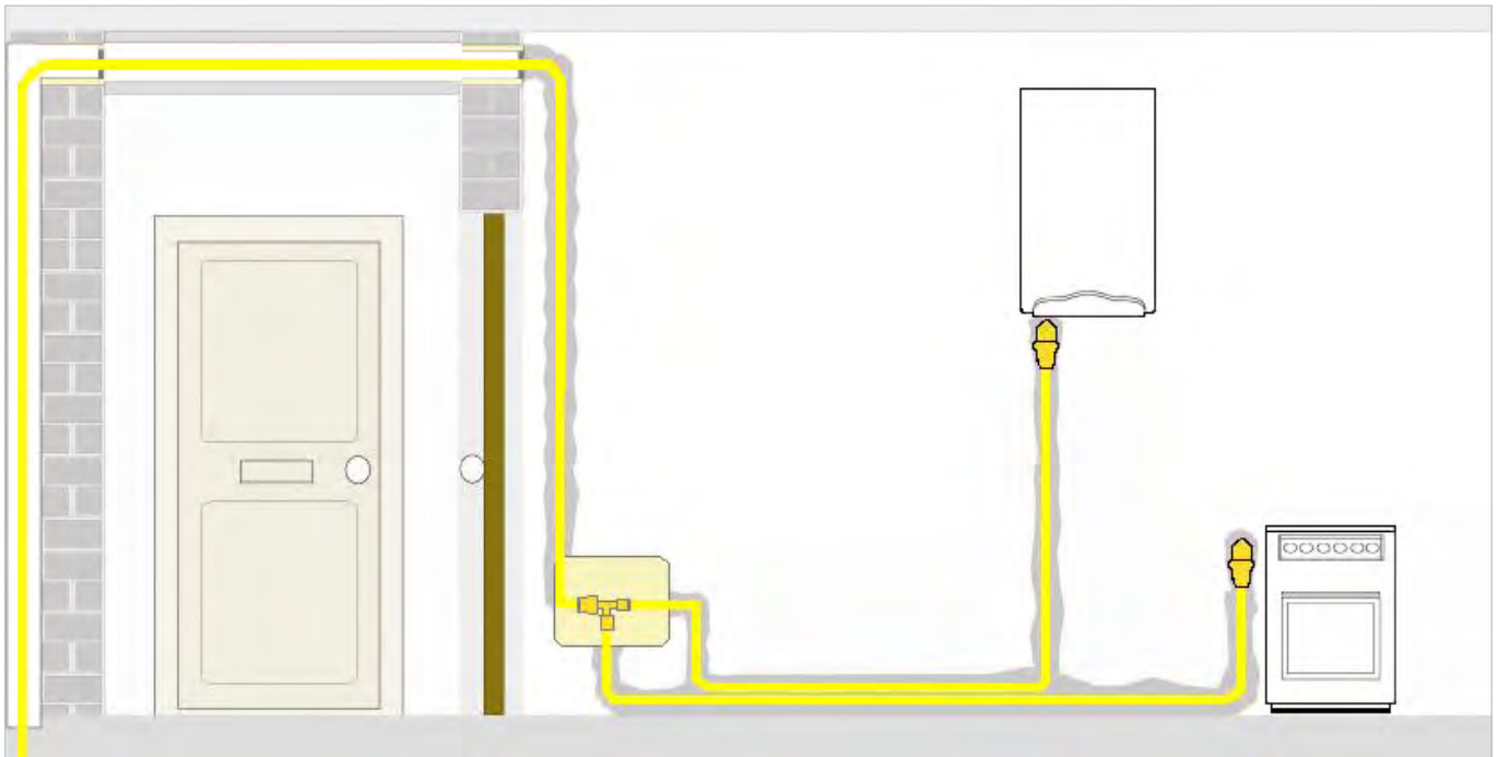
MULTIGAS SYSTEM
